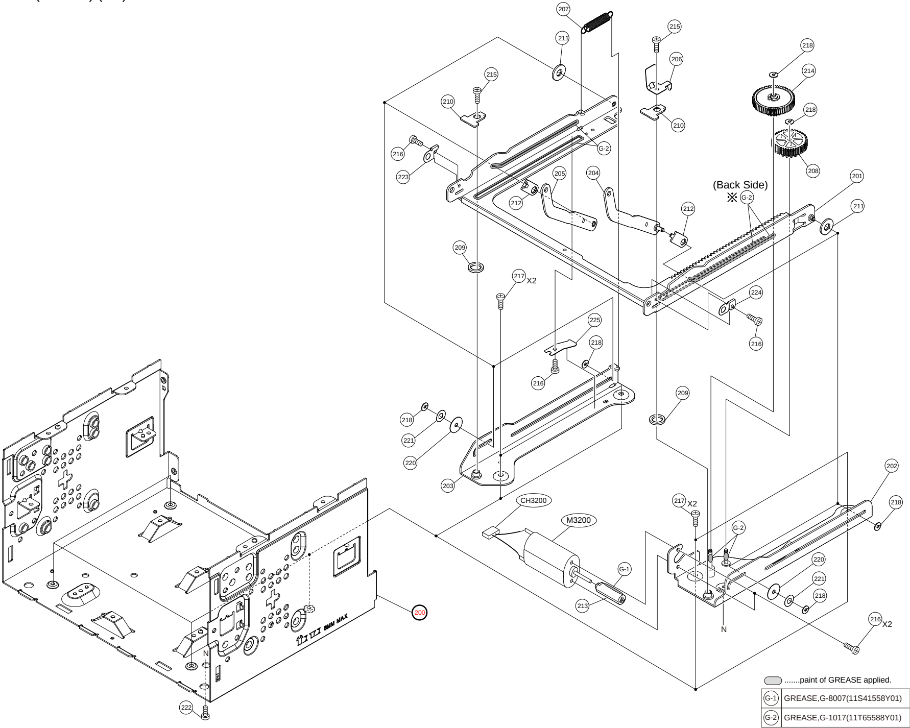
Exploded View (Cabinet) (5/5)
