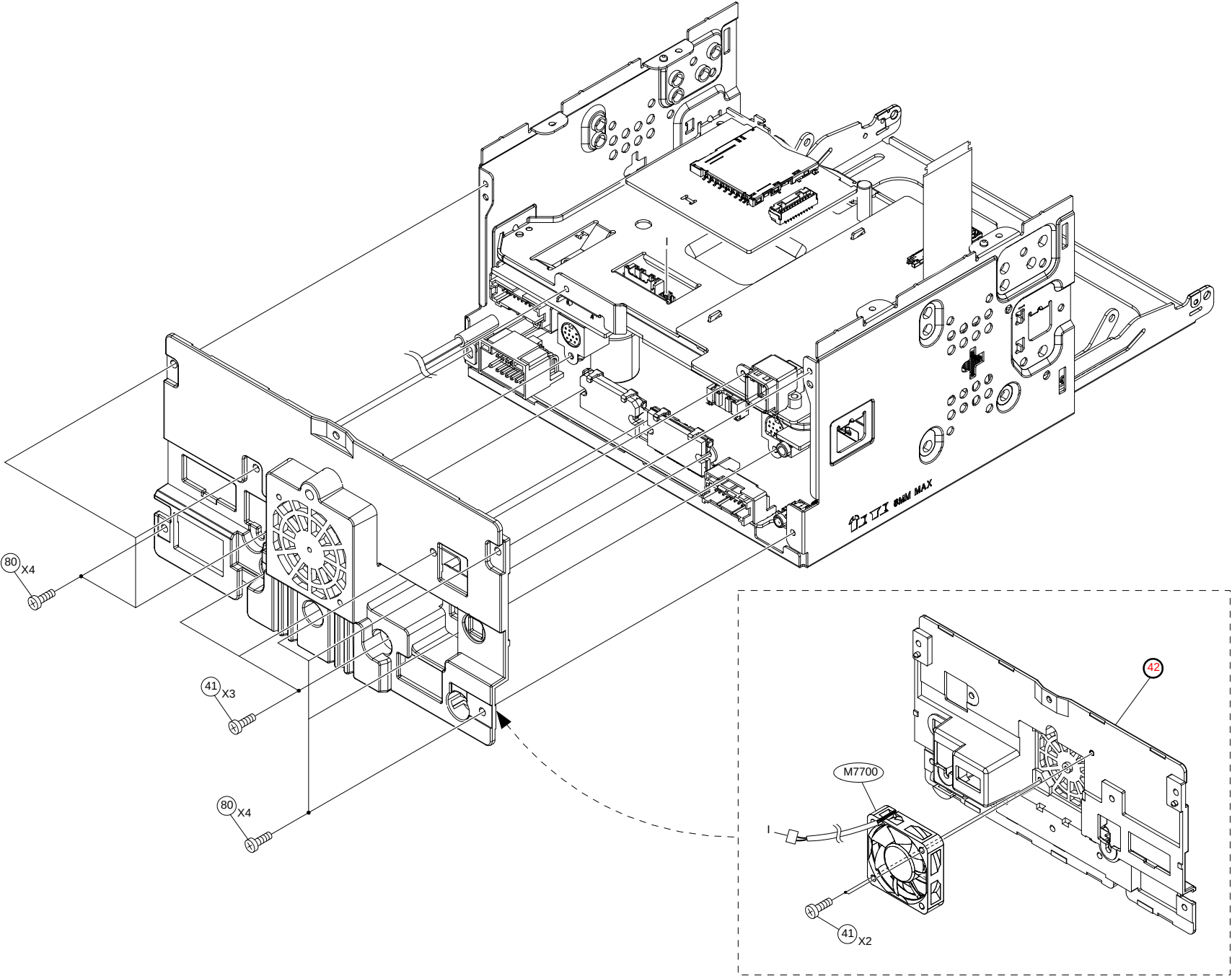
Exploded View (Cabinet) (2/5)
