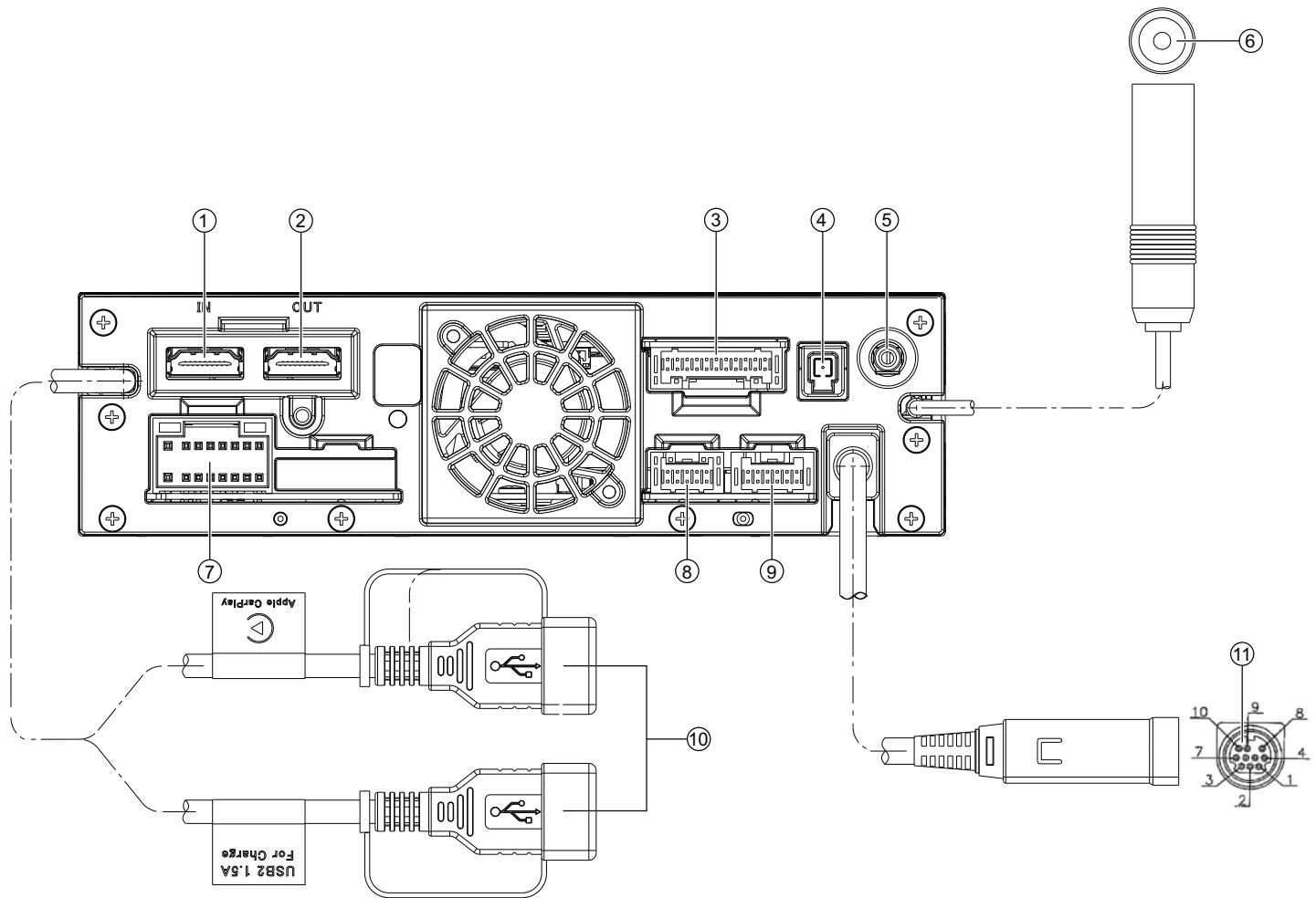
③ *CB6000(CAMERA CONNECTOR : SOC-P.W.Board) WTB,SM22B-PUDK-D -EK (09-38369Z03)
