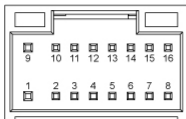
*CB3100 : WTB,F169B001-16
