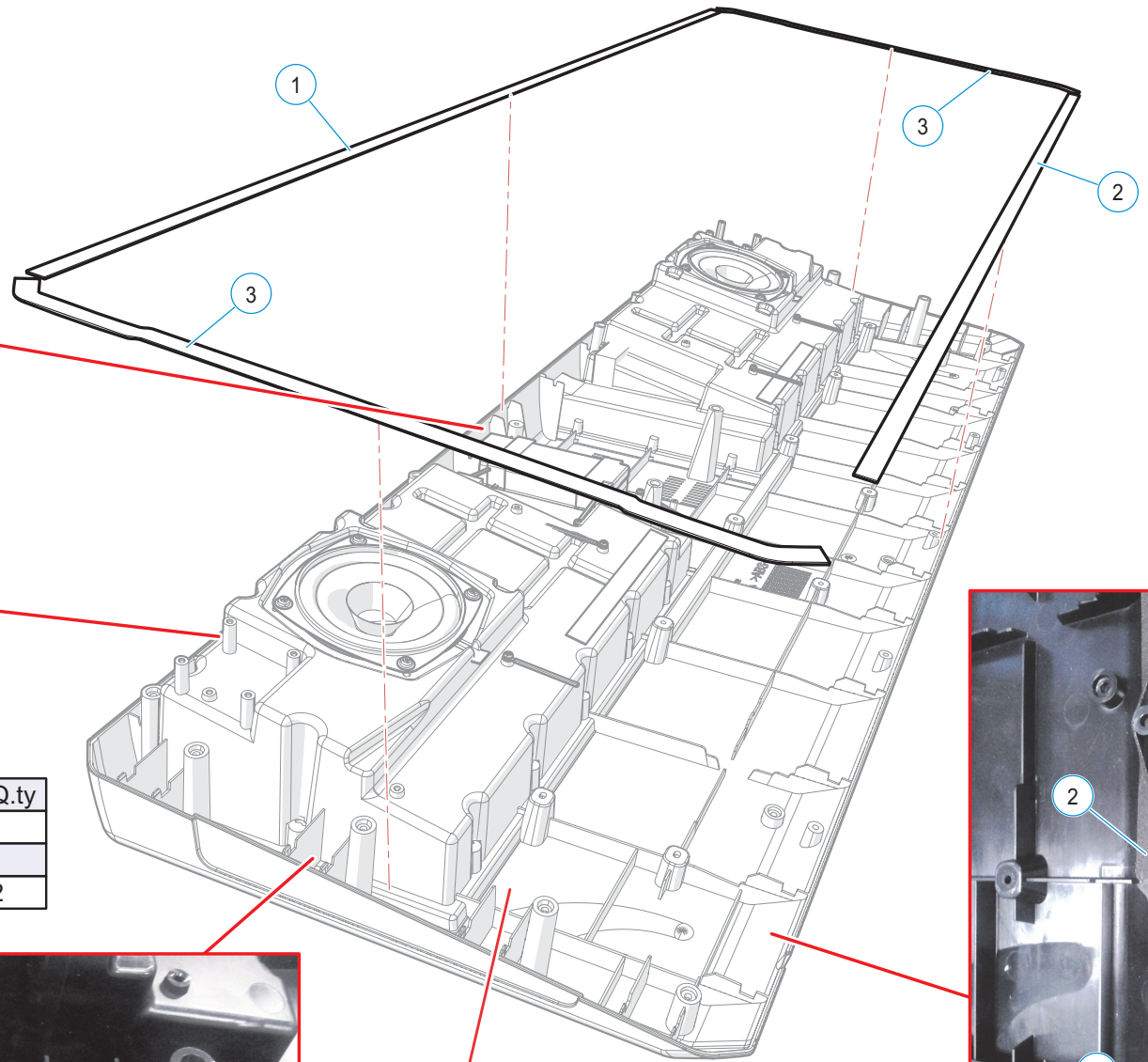
Lower Case Disassembly 1
