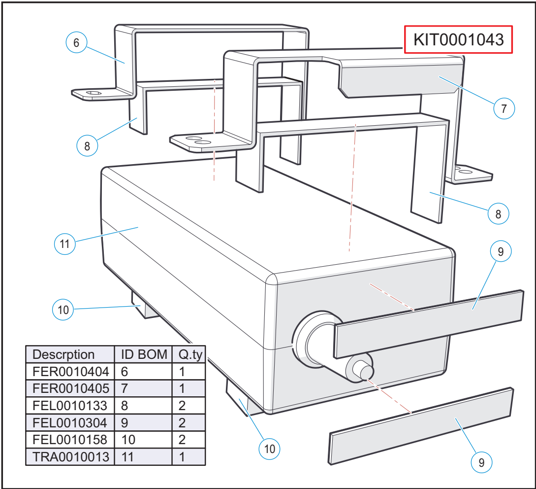
Lower Case Disassembly 3
