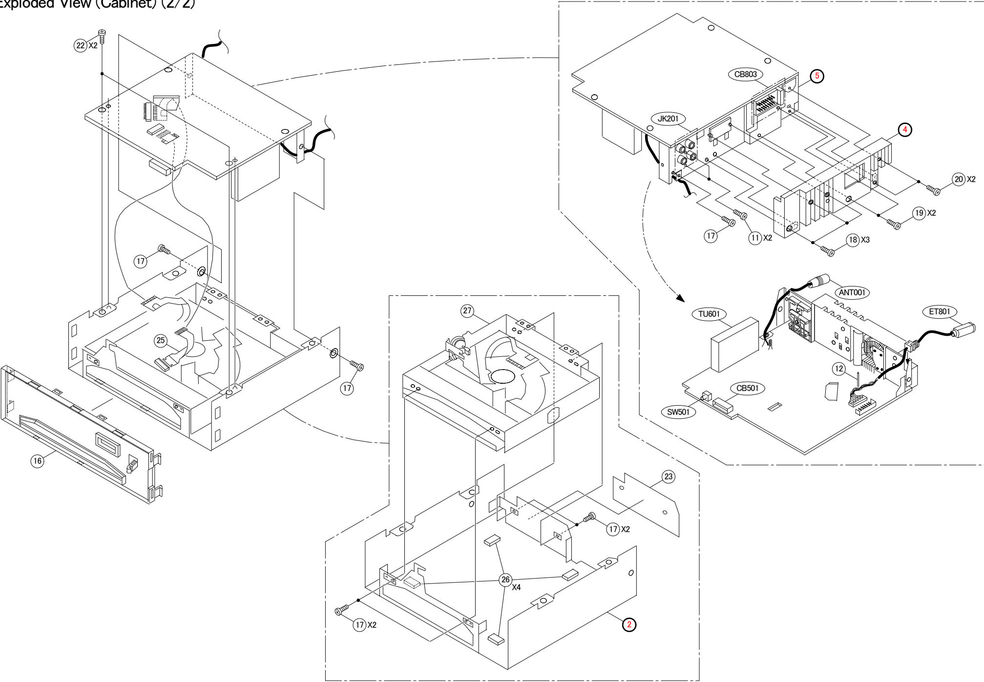
Exploded View (Cabinet) (2/2)
