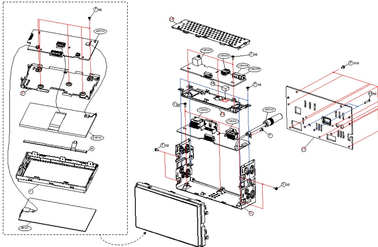
Exploded View (Cabinet)
